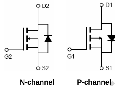
Schematic diagram
